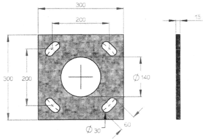
BASE PLATE DETAIL SCALE 1 : 8
